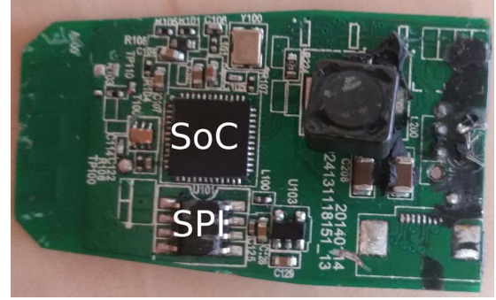
Figure 4. Philips Hue board
